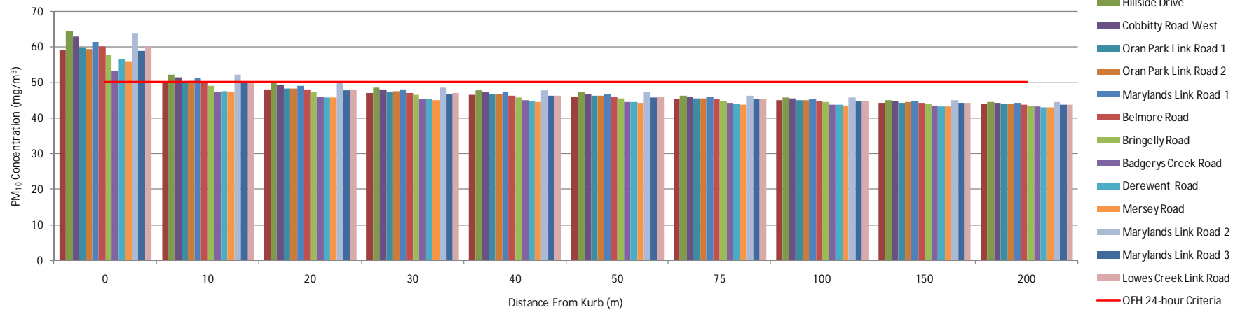
2026 AM Peak Maximum 24-hour PM 10 Concentration
