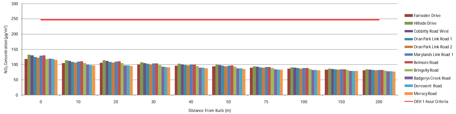
2016 PM Peak Maximum 1-hour NO 2 Concentration
