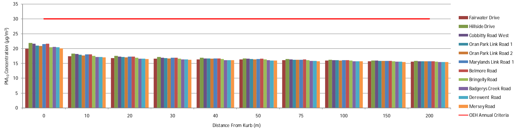
2016 PM Peak Annual PM 10 Concentration
