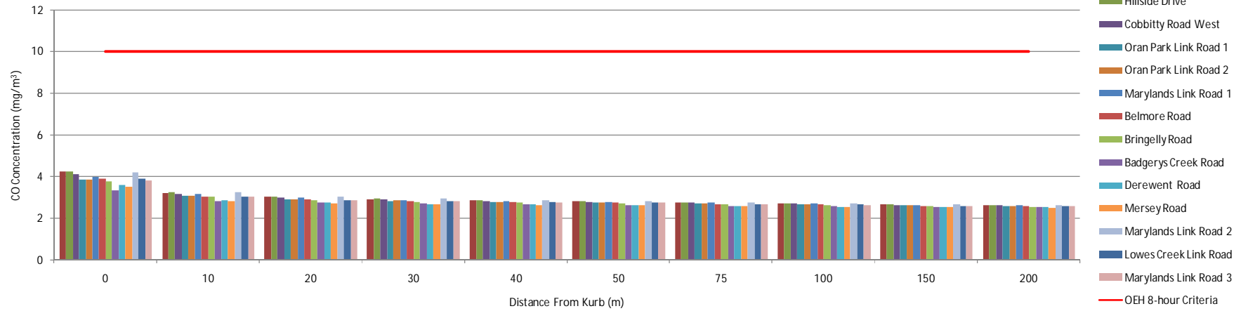
2026 AM Peak Maximum 8-hour CO Concentration
