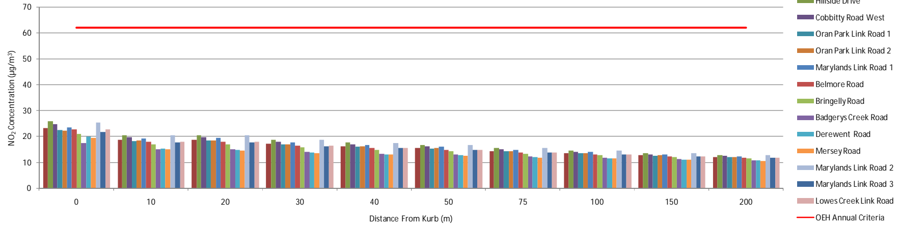
2026 AM Peak Annual NO 2 Concentration
