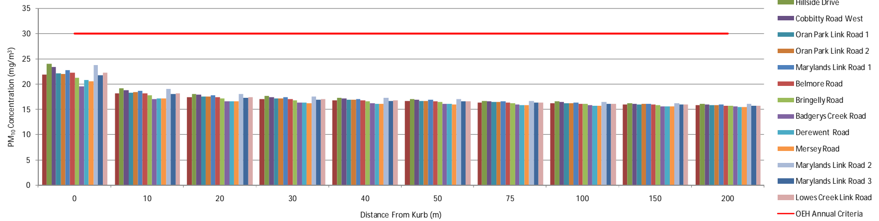
2026 AM Peak Annual PM 10 Concentration
