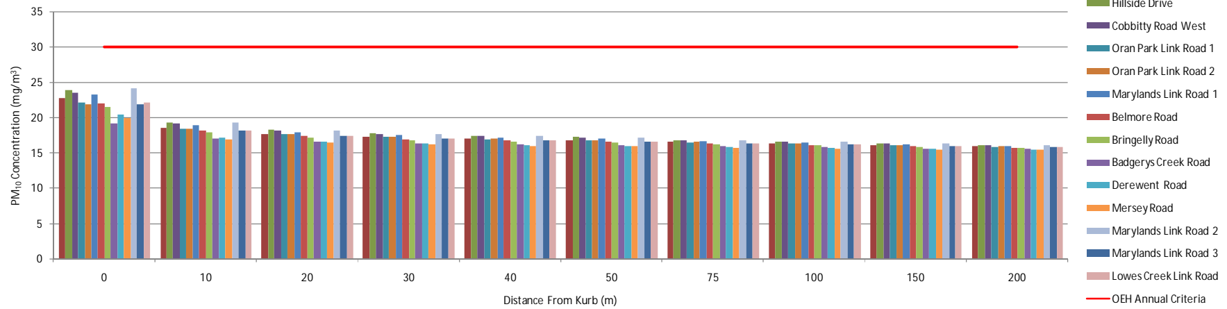
2026 PM Peak Annual PM 10 Concentration
