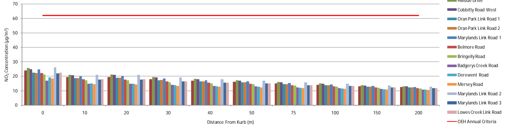
2026 PM Peak Annual NO 2 Concentration
