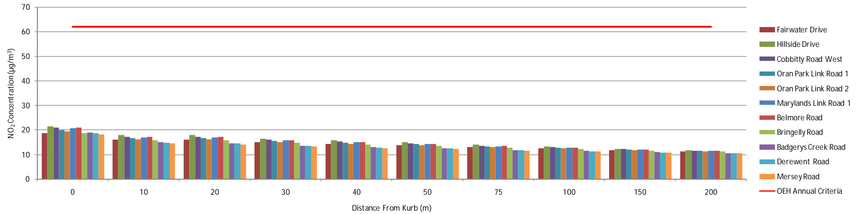
2016 PM Peak Annual NO 2 Concentration
