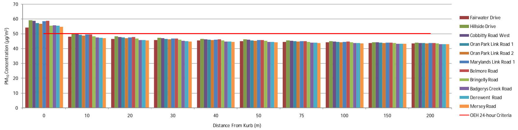
2016 PM Peak Maximum 24-hour PM 10 Concentration
