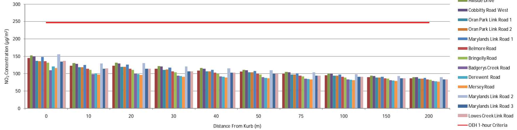
2026 PM Peak Maximum 1-hour NO 2 Concentration
