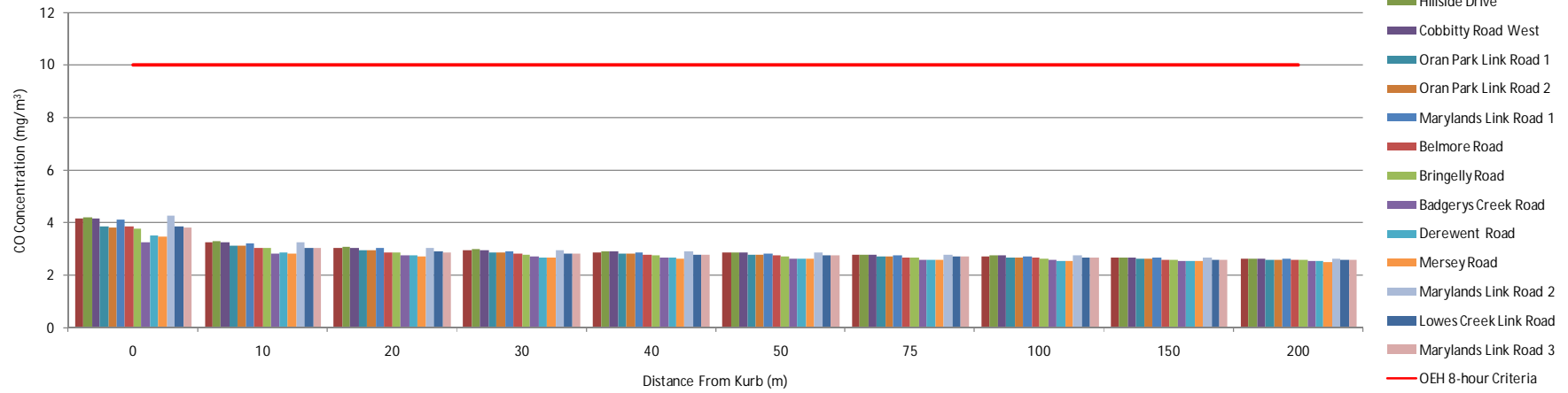
2026 PM Peak Maximum 8-hour CO Concentration
