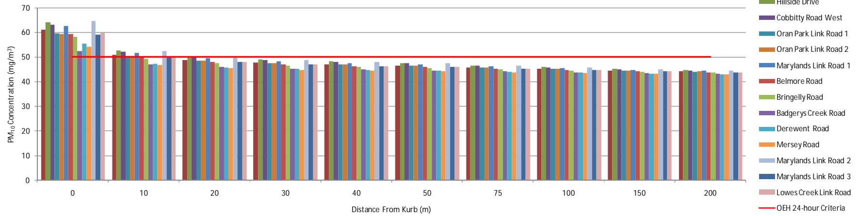
2026 PM Peak Maximum 24-hour PM 10 Concentration
