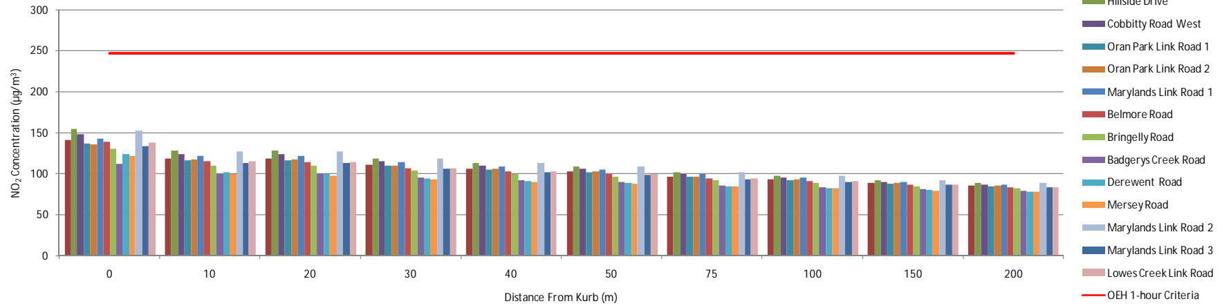
2026 AM Peak Maximum 1-hour NO 2 Concentration
