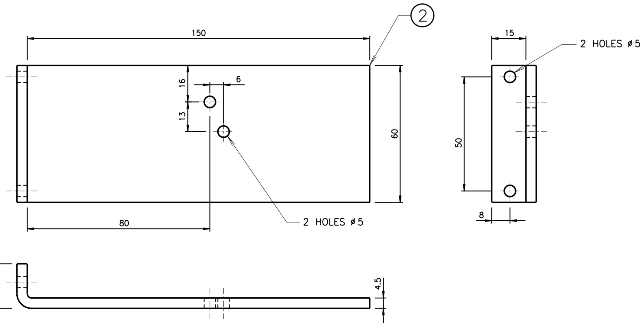
ITEM 2, FUSE HOLDER MOUNTING BRACKET MATERIAL: LEXAN EXELL D POLYCARBONATE SCALE 1:1
