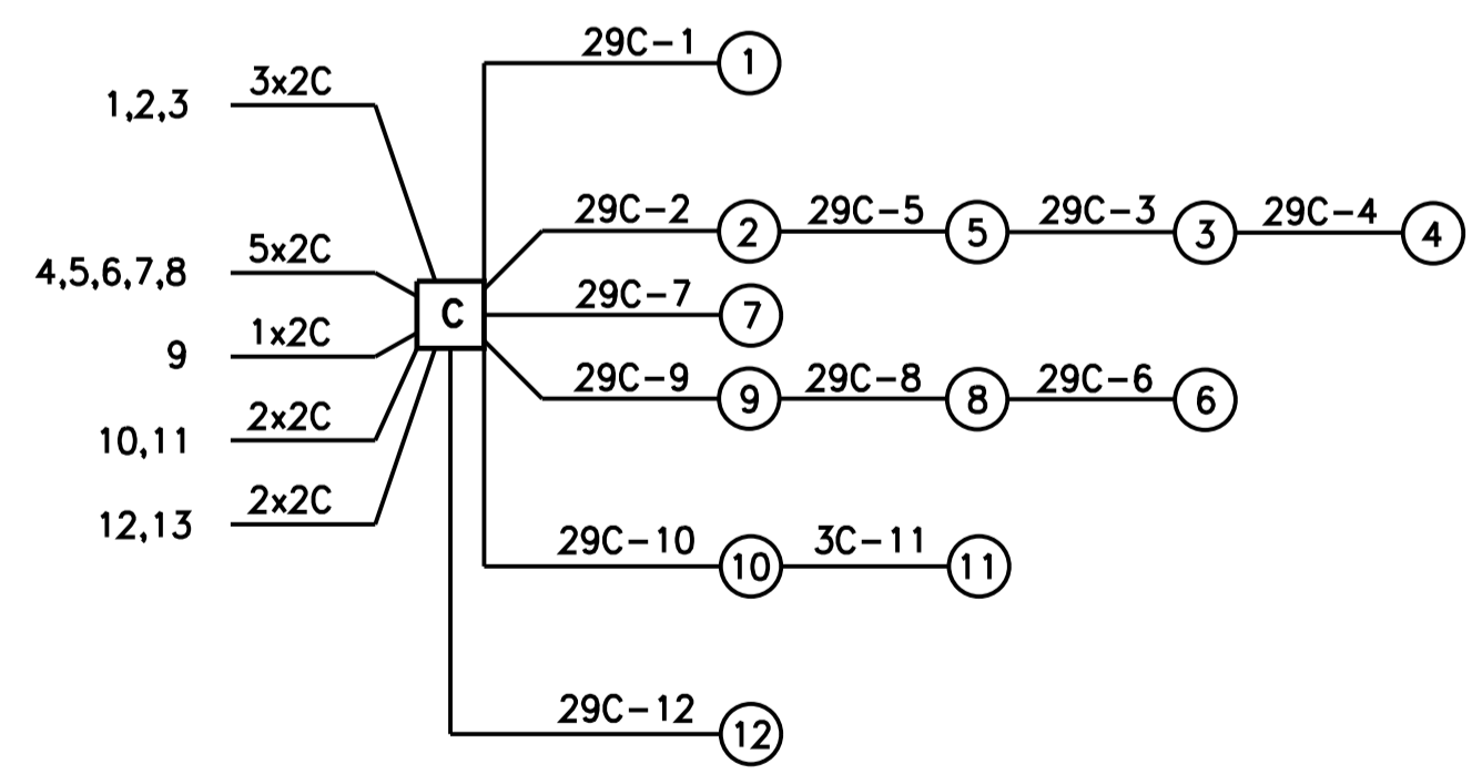
TYPICAL CABLE LAYOUT
