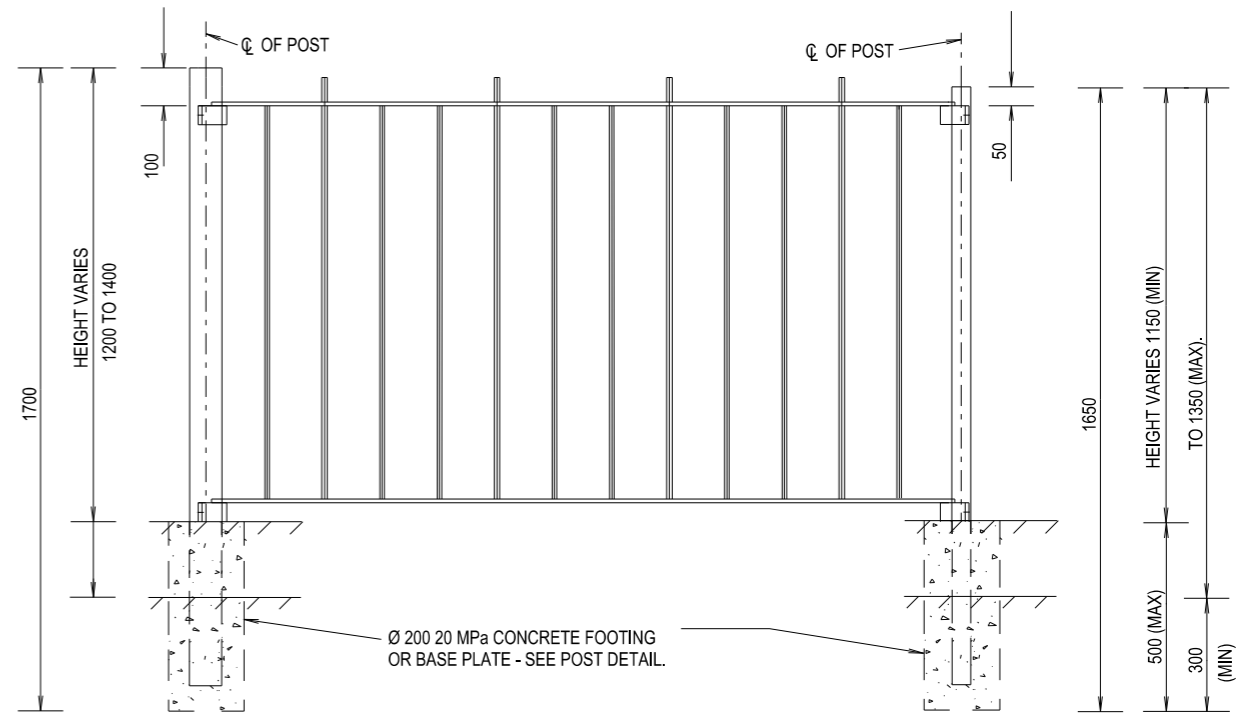
INTERMEDIATE POST
